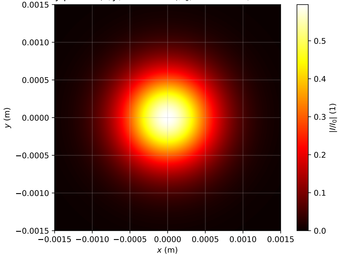
Intensity profile I(x, y, z = 2.866m)/I_0 , Pin=0.5Pcr, artificial time
